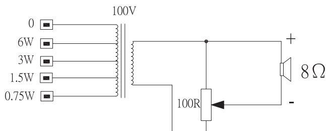
LB10-UC06V-x, circuitschema
